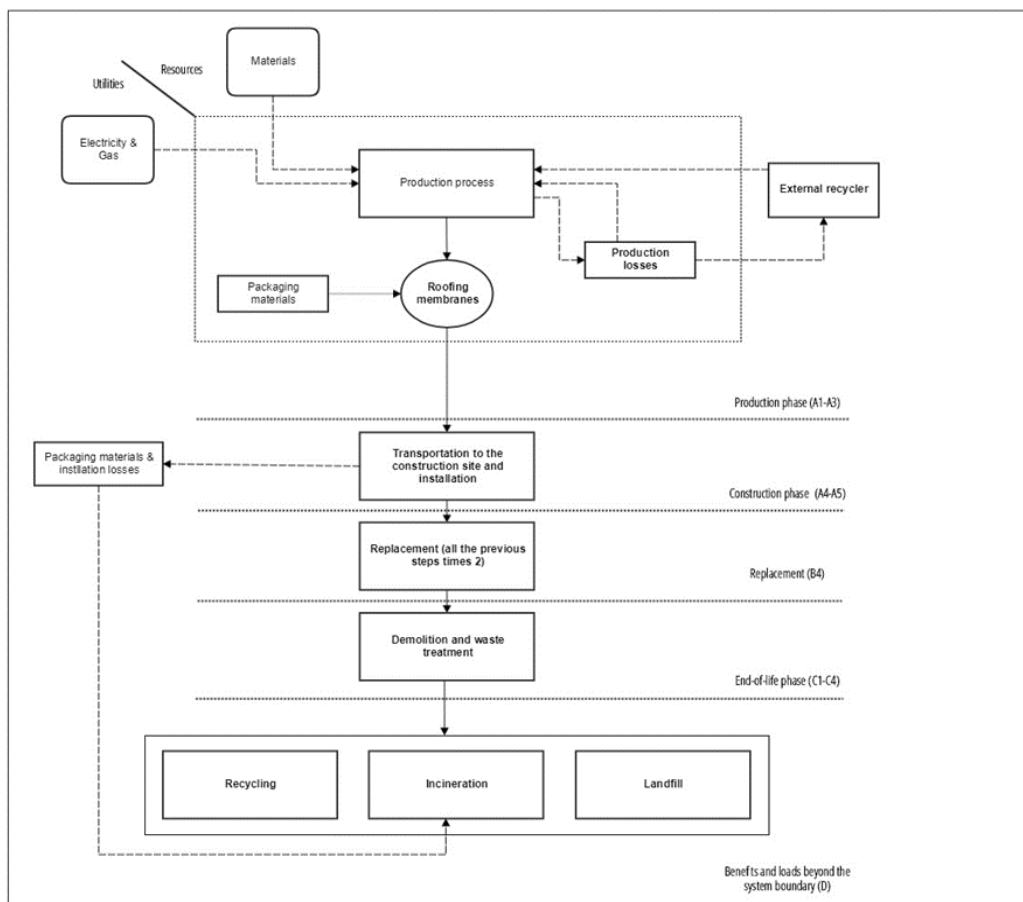
Figure 1: Process tree of one m² of Alkorplan A .
