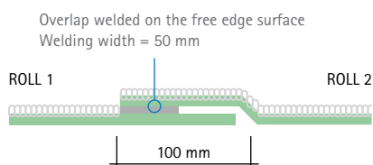
Welding sealing for longitudinal overlap.
