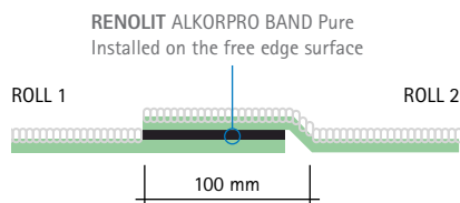
Butyl tape sealing for longitudinal overlap.
