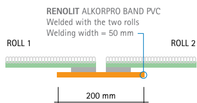
Welding sealing for transversal overlap.
